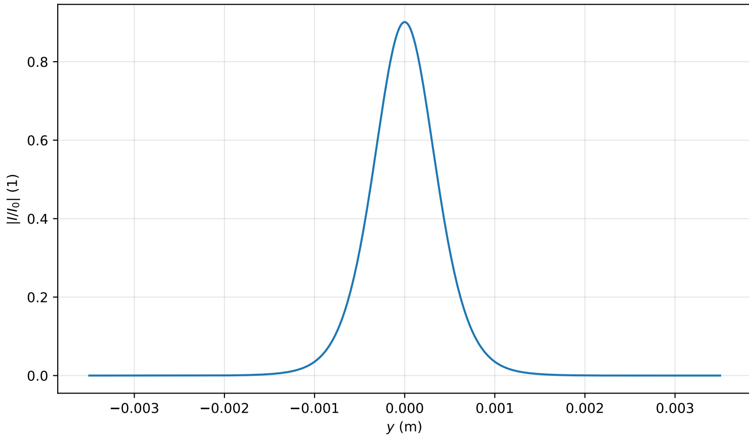
Intensity profile I(x=0, y, z=2.149)/I_0 , \text{Pin}=0.6P_{\text{cr}} , artificial time
